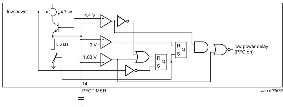
Fig 6. PFC switch on and switch off using the PFCTIMER pin
